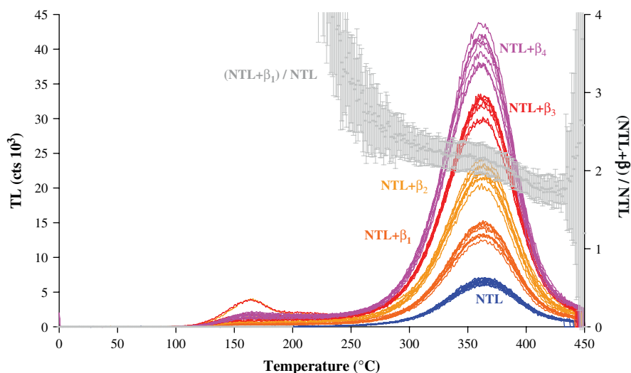
Fig. 4. Glow curves (natural and additive) and heating plateau (NTL + β/NTL) for sample EVA-LUM-06/7.
